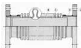
DU400 (DU400SG 附設限螺桿)
